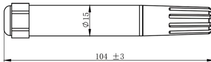
LFH51 Dimensions
